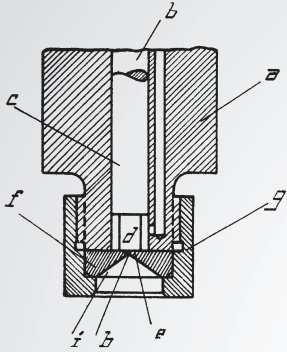
Nozzle needle with flattened pinpoint
