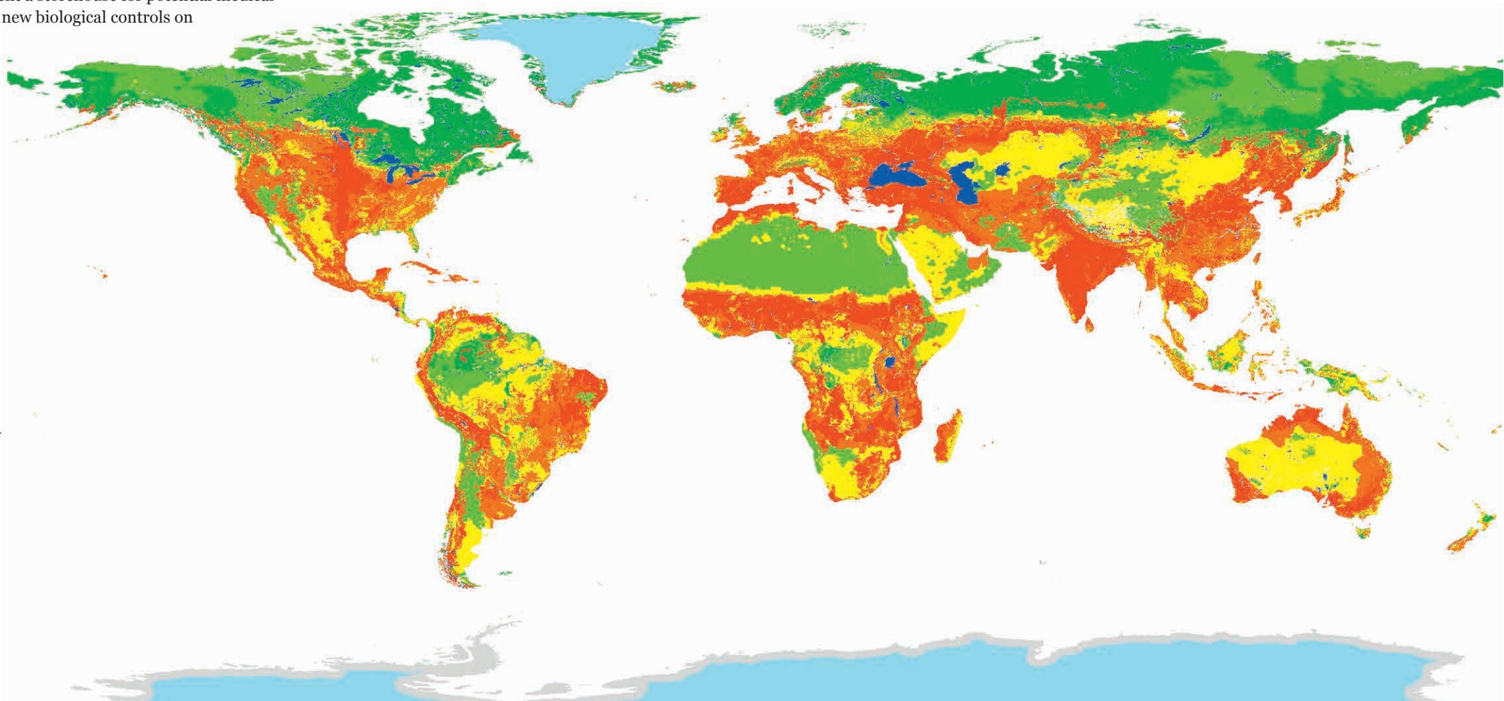
Figure 6: Global map showing the distribution of potential threats to soil biodiversity All datasets were harmonized on a 0-1 scale and summed, with total scores categorized into five risk classes (from very low to very high) 22 .
