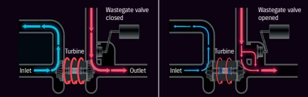
Wastegate valve
