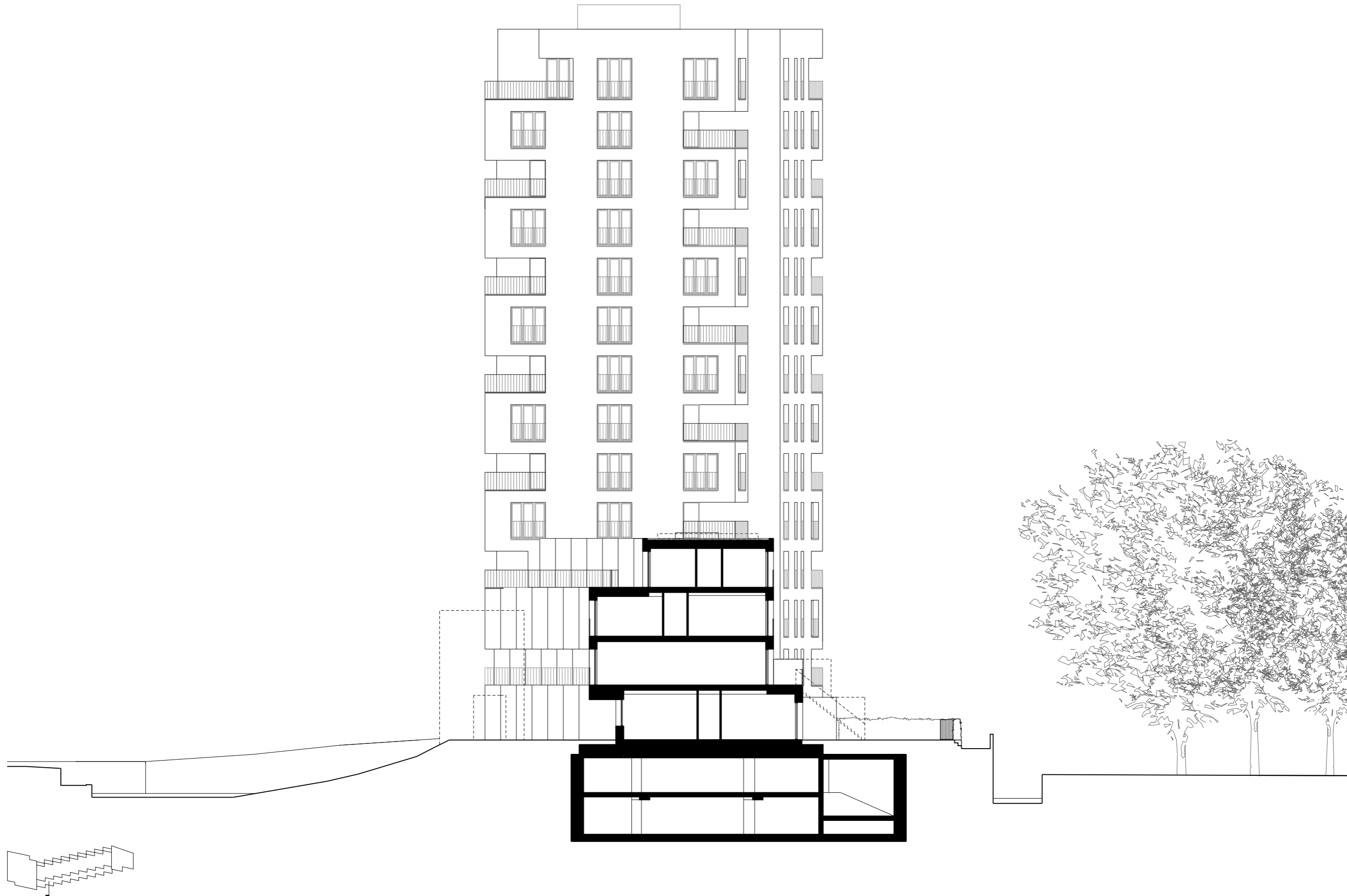
Townhouse section (1:250)
